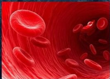
Atmospheric Oxygen
